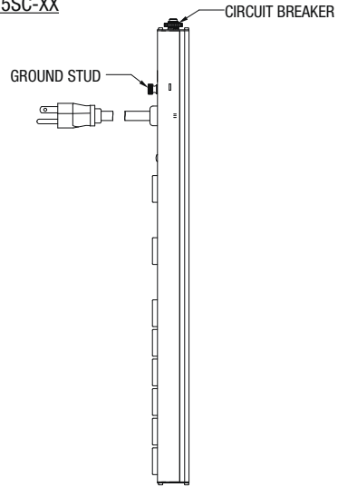
PD-815SC-XX
